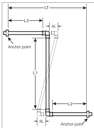
Z-Type Offset
