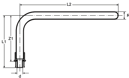
PureFlow Press 90° Stub-out Brazed Copper P x FTG - Model 2820.1ZL
