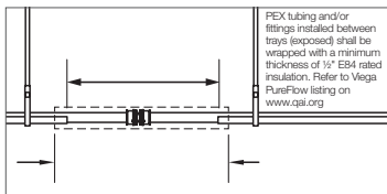
Plenum installation
