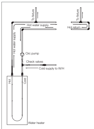
Typical domestic hot water circulation piping
