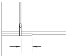
Hanger to end of tray
