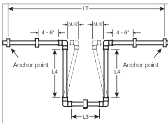
U-Type Looped Offset
