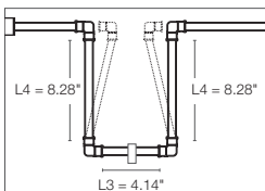
U-Type Expansion
