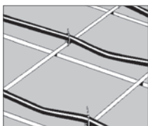
Tubing must be fastened to the reinforcing mesh on rebar with the use of plastic zip ties
