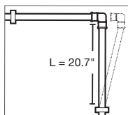
Corner Expansion Example
