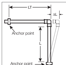
Corner Offset
