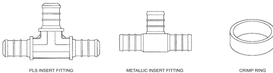
FIGURE 3—VIEGA PureFlow CRIMP FITTINGS
