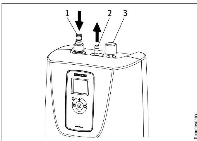
Plumbing connections
