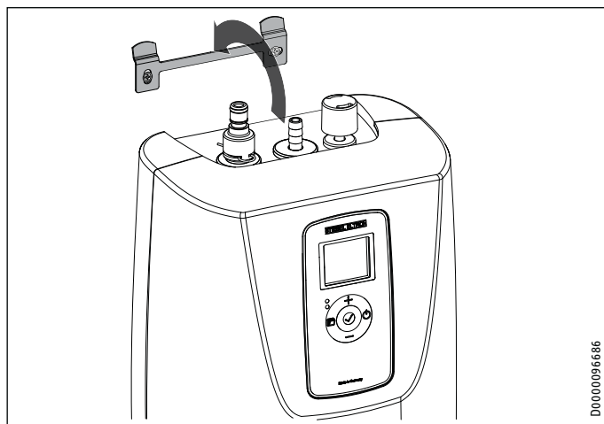
1 Mounting the UltraHot Plus/Premium
