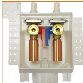
Washing Machine
