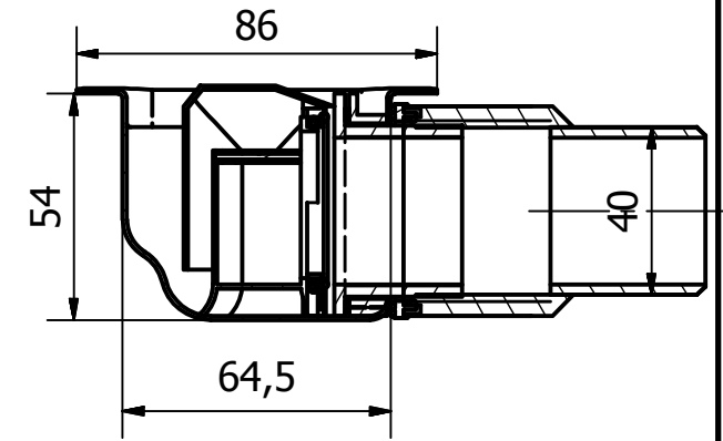
A'-A' ( 1/2 )
