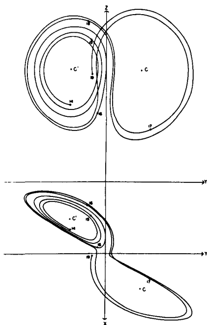
THE FIRST STRANGE ATTRACTOR. In 1963 Edward Lorenz could compute only the first few strands of the attractor for his simple system of equations. But he could see that the interleaving of the two spiral wings must have an extraordinary structure on invisibly small scales.
