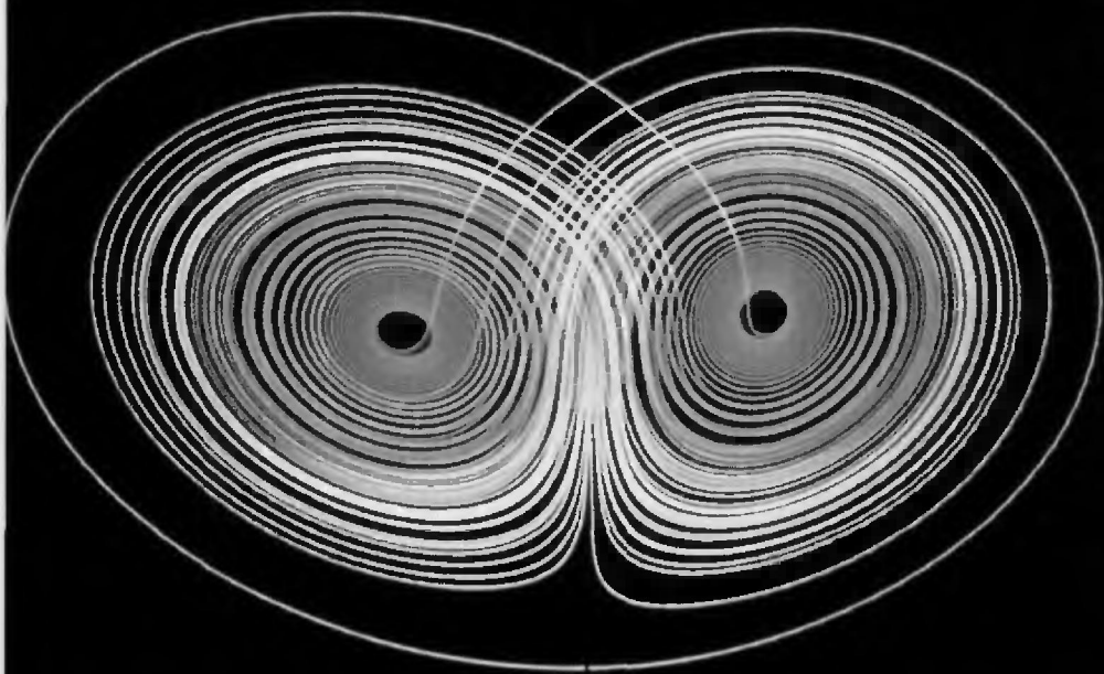
THE LORENZ ATTRACTOR.
