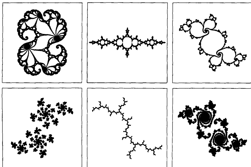
AN ASSORTMENT OF JULIA SETS.
