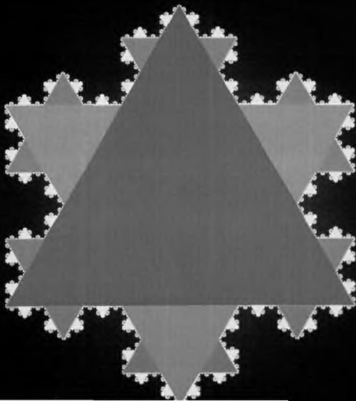
THE KOCH CURVE.
