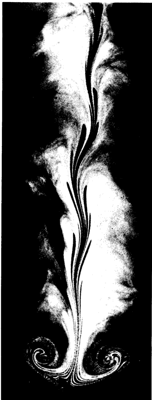
CHAOTIC FLOWS. A rod drawn through viscous fluid causes a simple, wavy form. If drawn several times, more complicated forms arise.
