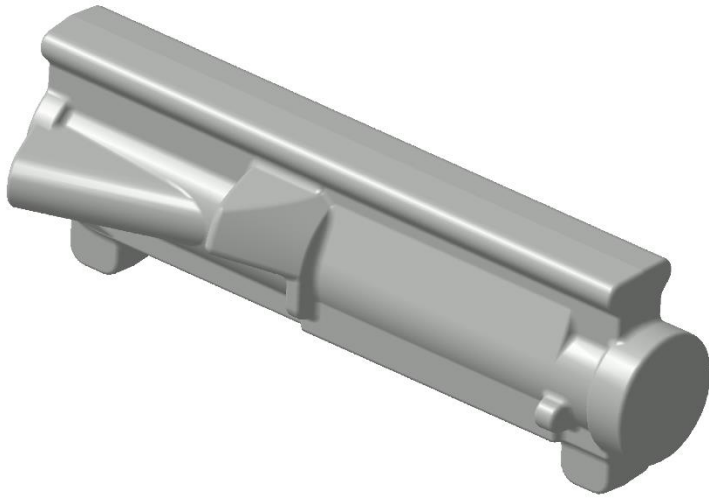
CAD MODEL RAW FORGING
