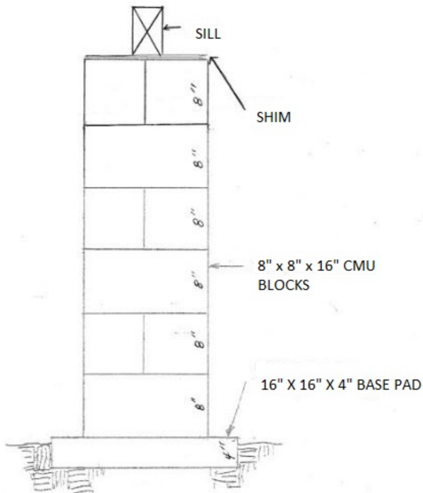
TYPICAL 6 BLOCK PIERS
