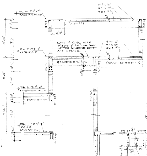
ELEVATOR SECTION SCALE 3/8" = 1'-0"
