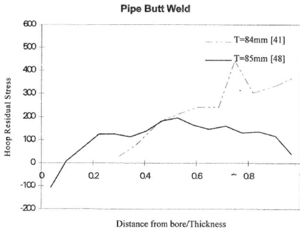
Figure 4 Comparison of through-thickness hoop residual stress distributions in girth welded pipes of various thicknesses (Bate et al, 1997).
