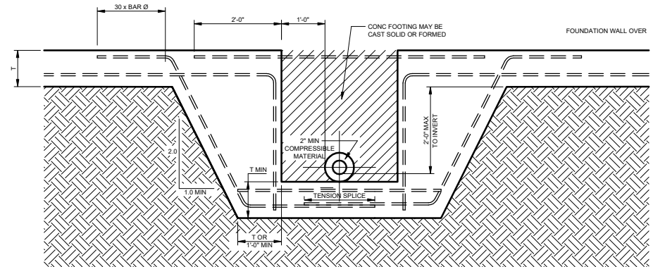
SERVICE PIPES BELOW FOOTING ELEVATION SCALE: NTS
