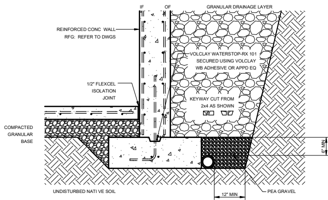
TYP STRIP FOOTING INTERSECTION SCALE: NTS
