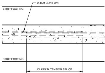
TYP STRIP FOOTING ARFG SPLICE SCALE: NTS
