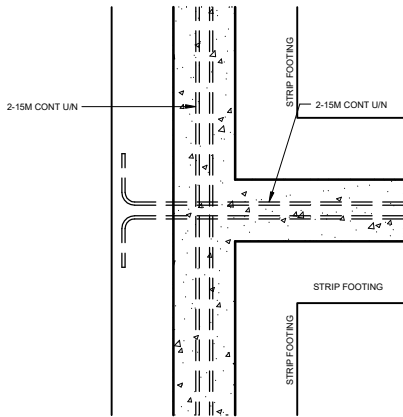
TYP STRIP FOOTING INTERSECTION SCALE: NTS
