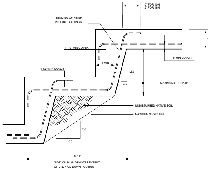
TYP STEPPED DOWN FOOTING SCALE: NTS T DENOTES FOOTING THICKNESS
