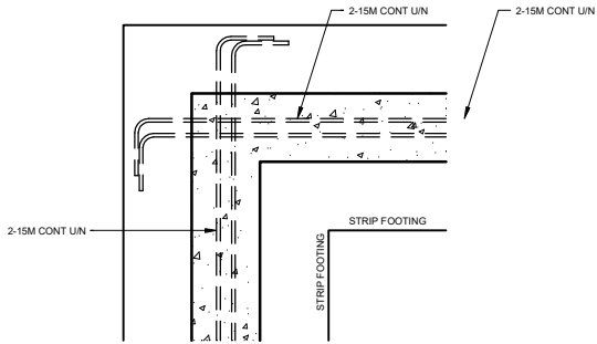
TYP STRIP FOOTING CORNER SCALE: NTS
