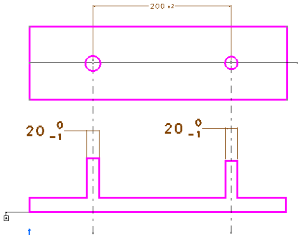
BOTTOM PLATE
