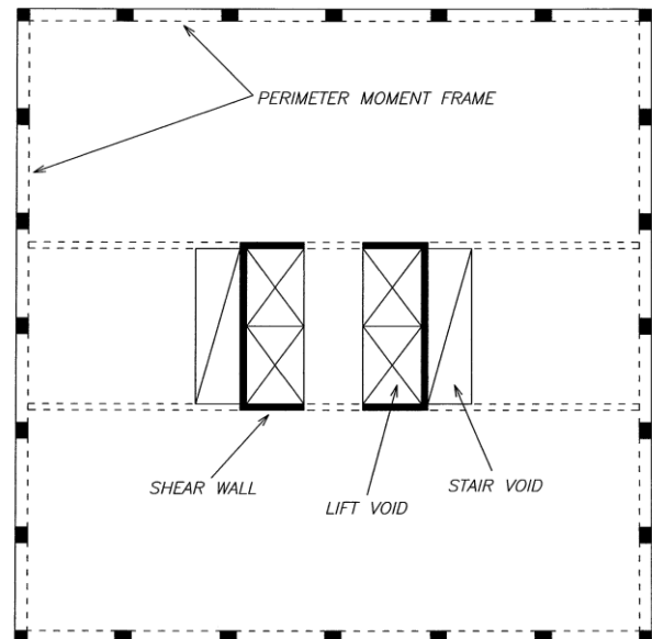
Figure 4: Voids surrounding shear core.
