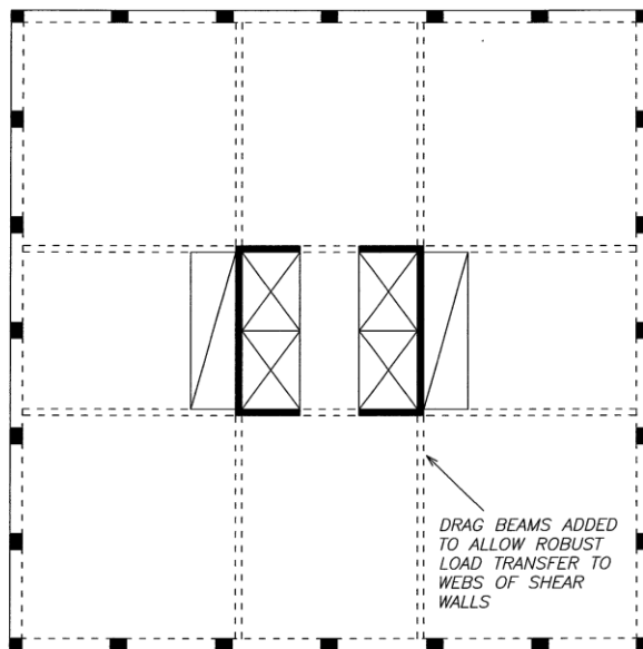
Figure 12: Diaphragm improvement using internal drag beams.
