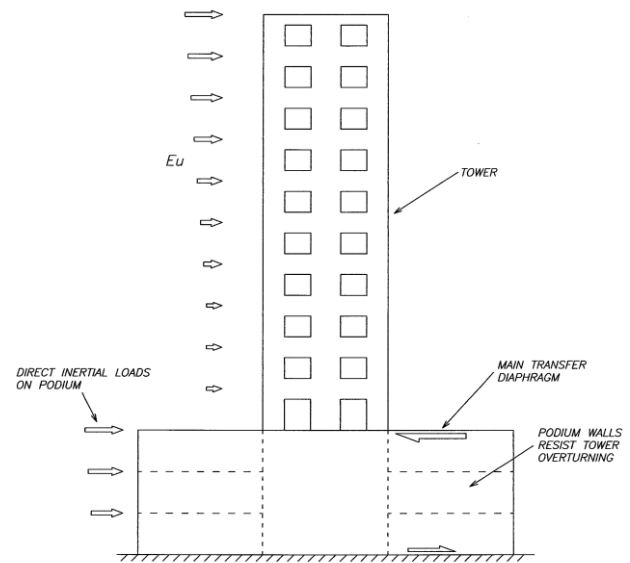
Figure 9: Transfer forces in towers with podiums.
