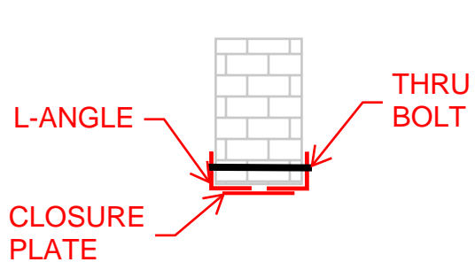
LINTEL SECTION
