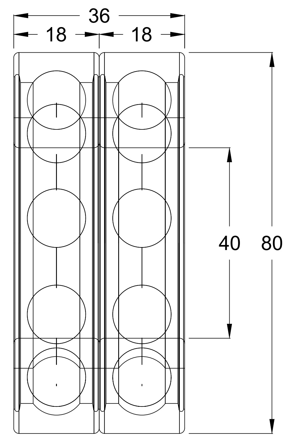
Bearing 6208 Bearing 6208
