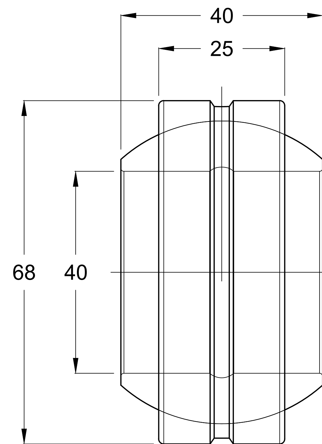
Bearing GEH40S
