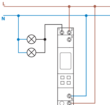
Type 12.71
