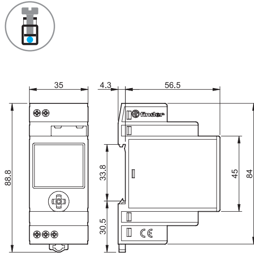
12.61 / 12.A1 Screw terminal
