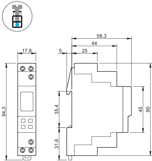
12.71 Screw terminal
