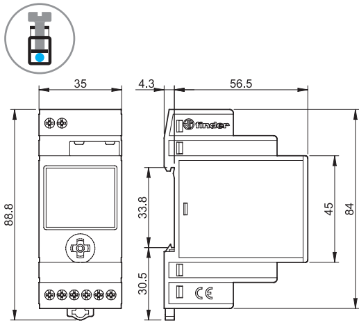
12.62 / 12.A2 Screw terminal
