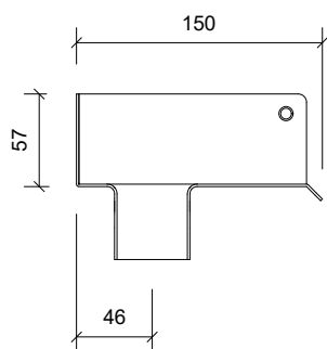
Snit/Section/Abschnitt
