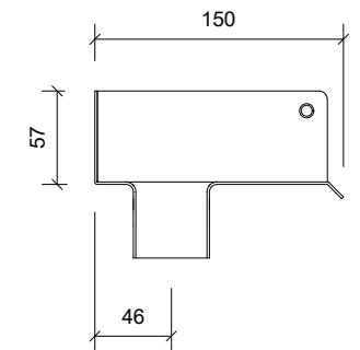
Snit/Section/Abschnitt
