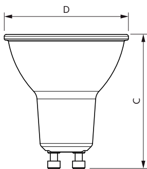
LED SceneSwitch 50W GU10 WW 36D RF ND SRT4
