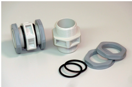
Joining accessories enable cables to be run between 2 cabinets.
