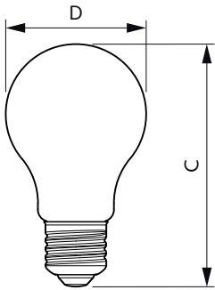
LEDbulb ND 10-75W A60 E27 827 2CT
