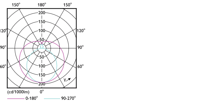
Light Distribution Diagram
