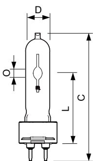
MASTERColour CDM-T Elite 70W/930 G12 1CT/12
