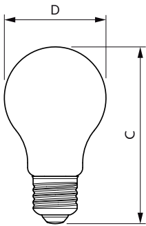
MASTER VLE LEDBulbD3.4-40W E27 927 A60 CL G
