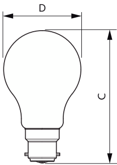
MAS LEDBulb DT5.9-60W B22 927A60CL G
