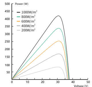
Power-Voltage Curve(420W)
