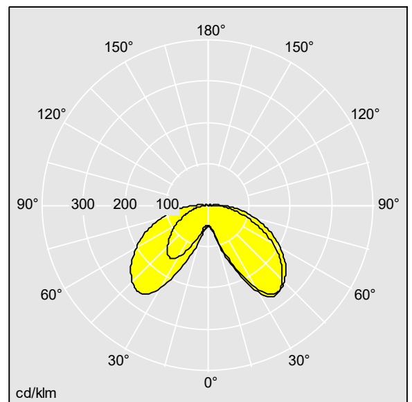
TL_AVFR18L35WST730.ltd
