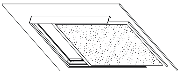
Fig.5 - Slide in the panel ensuring the cables and driver do not get caught or pinched.
