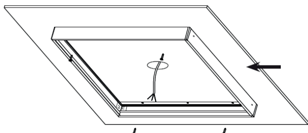
Fig.3 - With the supply cable in position, mark the location of the 4 frame fixing holes. Fix in to position using suitable fixings and screws ensuring secure.
