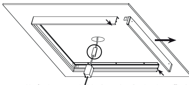
Fig.4 - Unclip the one end of the frame (not fixed to the ceiling). Terminate the supply cable to remote driver using suitable connector/junction box. See individual panel wiring instructions.
