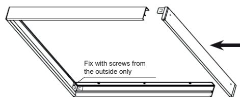
Fig.2 - Assemble the frame ensuring the correct orientation of the corners. The corners clip in to location to assist with assembly
