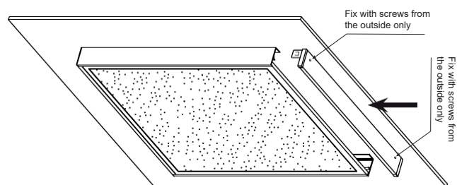
Fig.6- Refit the end panel until it clips in to position ensuring secure.
