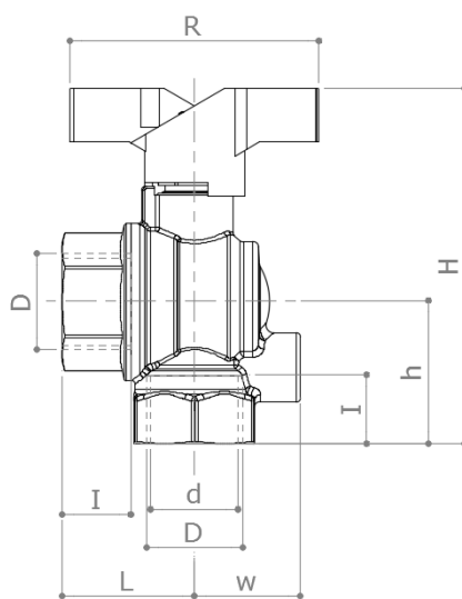
Size 3/4" and 1"
