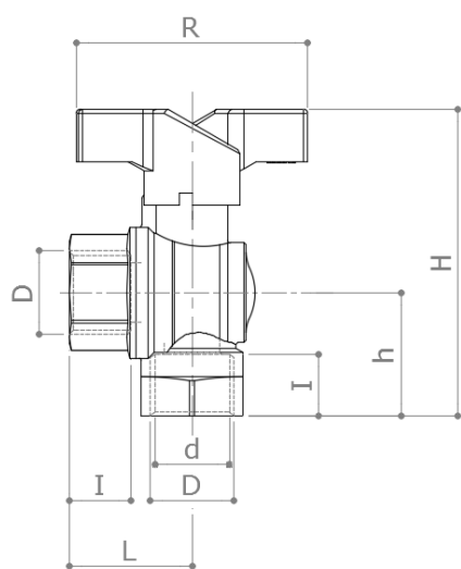
Size 1/2"
