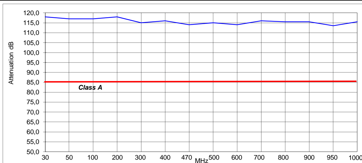
Screening Attenuation
