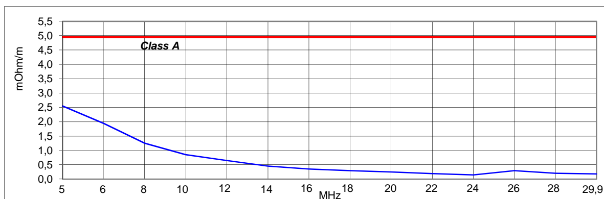
Screening Attenuation
