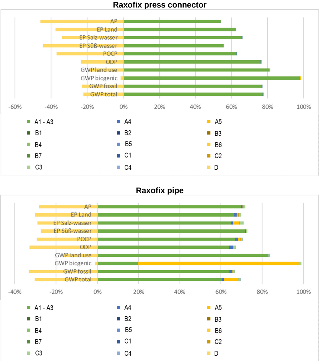
Illustration 3 Percentage of the modules in selected environmental impact indicators
