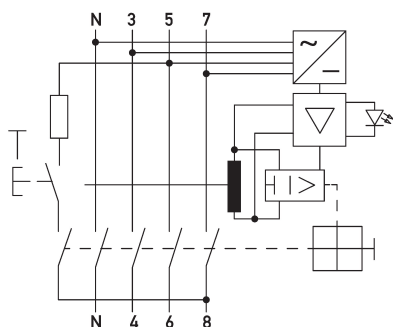
Wiring diagram
