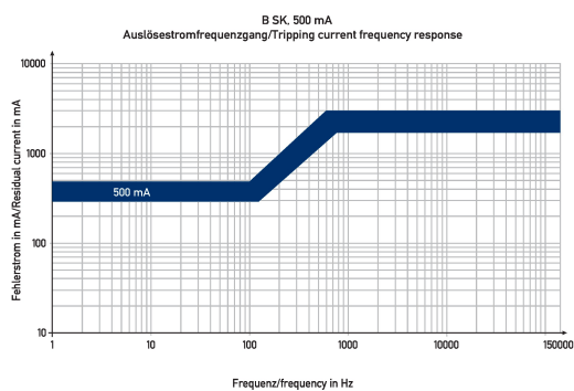
Characteristic B SK 500 mA
