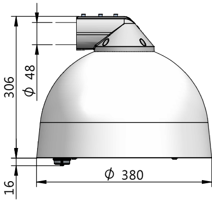
Cph LED / City gen2 BRS561 / 761 Side entry \varnothing 48\text{mm}
