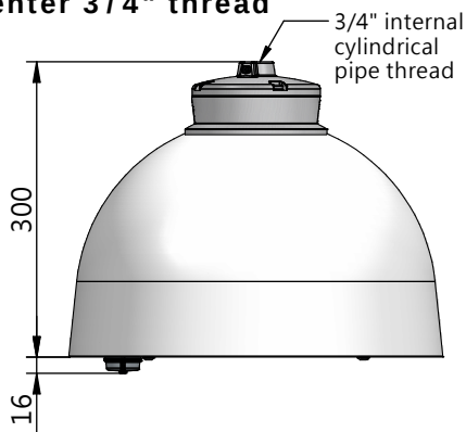
Cph LED / City gen2 BDS561 / 761 Center 3/4" thread
