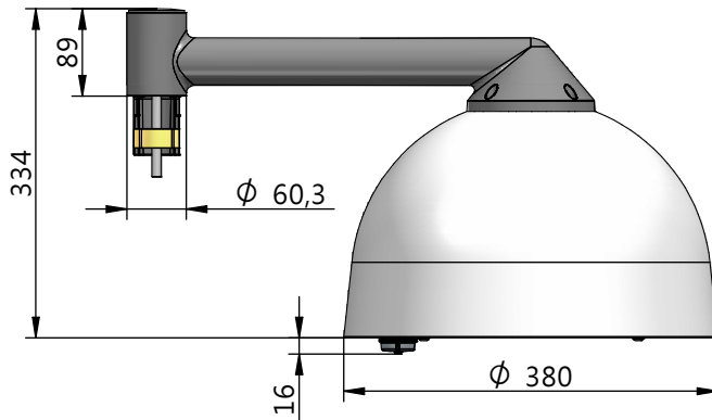
Cph LED / City gen2 BPS561 / 771 Post top \varnothing 60\text{mm}
