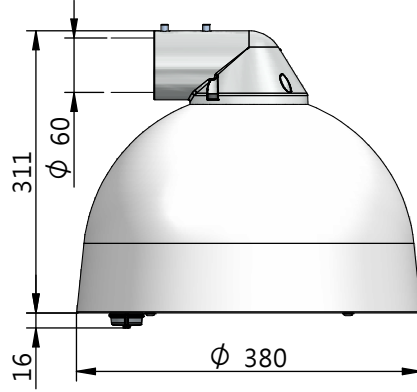
Side entry \varnothing 60\text{mm}
