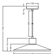
DECOR PLASTER WOOD PEND 320 E27WT
