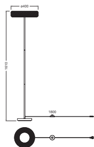
DECOR MESH FLOOR 18.5W 830 BK
