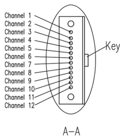
12 channels of MPO connector
