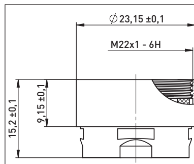
Clinic Snap NEOSTRAHL® Adapter STD M22x1
