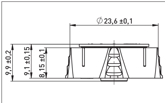
Clinic Snap NEOSTRAHL® STD Insert
