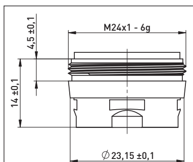
Clinic Snap NEOSTRAHL® Adapter STD M24x1
