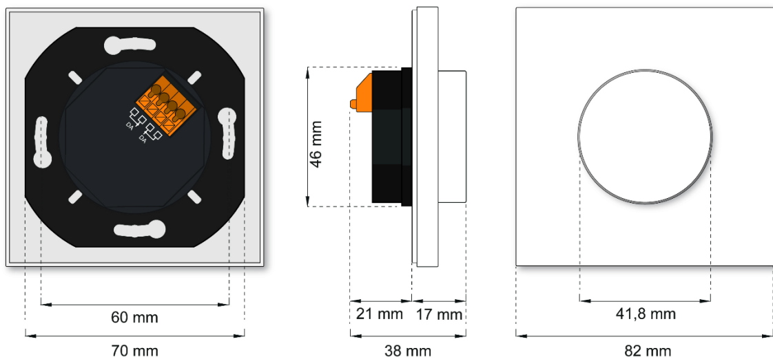
dimensions DALI-2 Rotary Touch with cover
