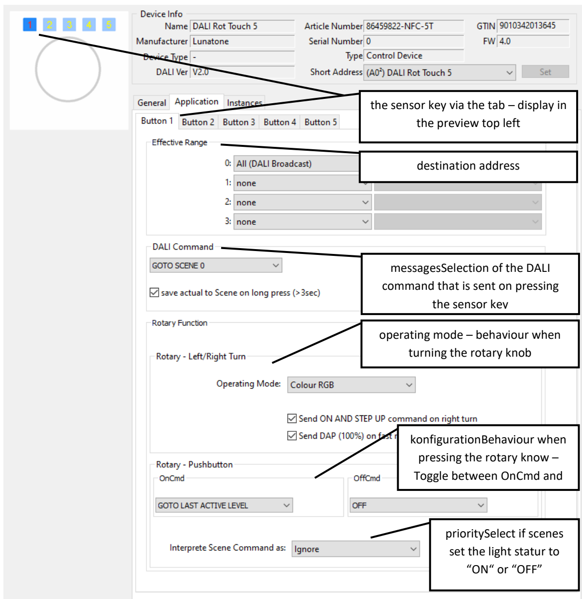
Figure 3. DALI Cockpit: configuration of the application – Tab: “Application”
