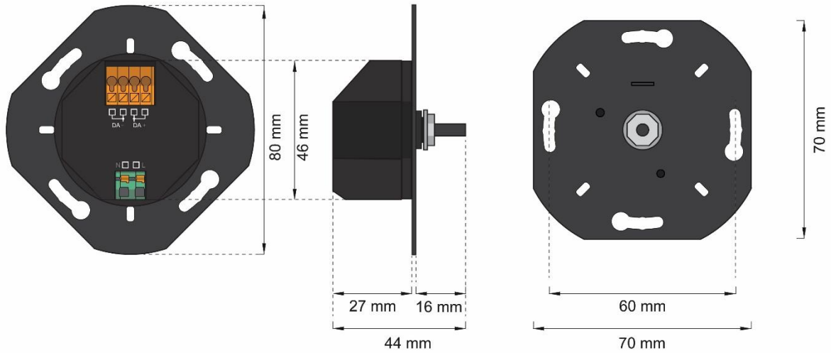
dimensions DALI-2 ROT Touch PS
