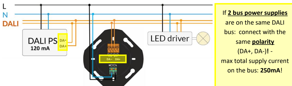
Figure 1. Installation Example DALI-2 ROT Touch PS with additional DALI PS on the DALI Bus
