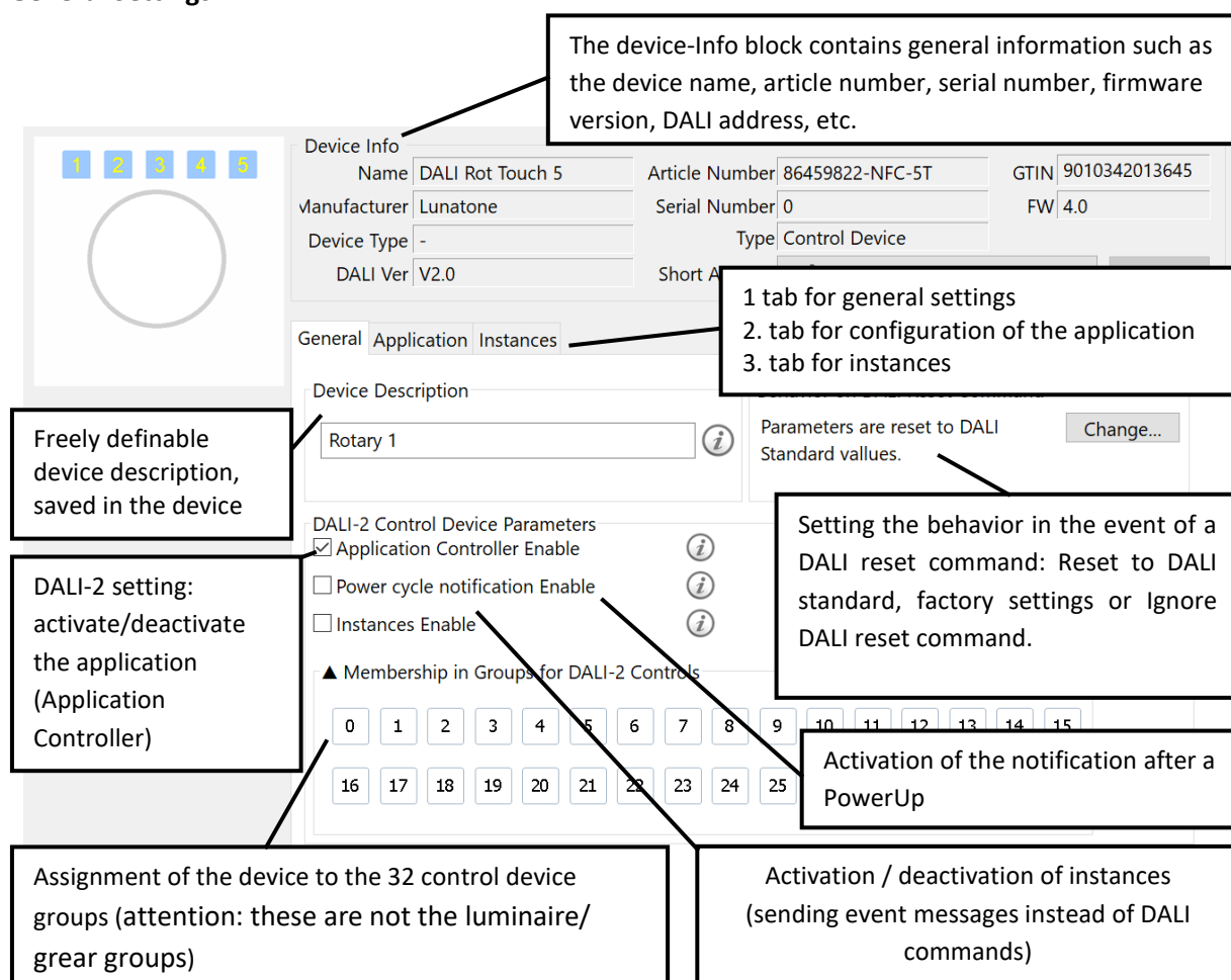
Figure 2. DALI Cockpit: general Configuration options – Tab: “General”
