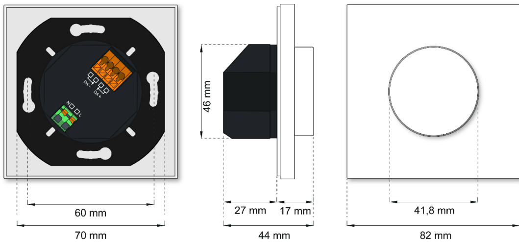
dimensions DALI-2 ROT Touch PS with cover
