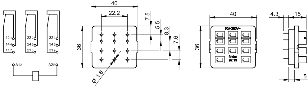
62.3x plug on 92.13 is 63.3 mm high
