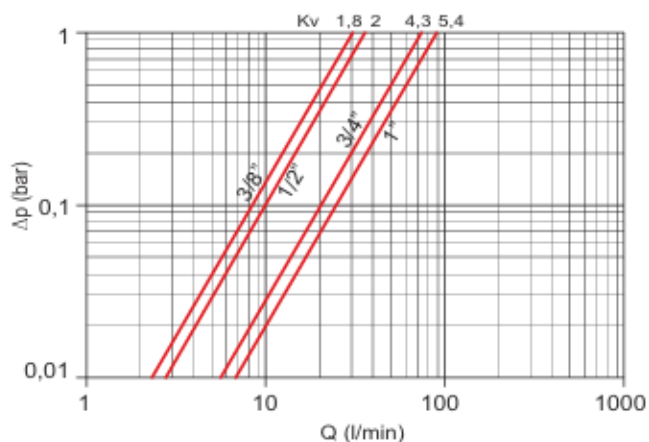
Flow/pressure drop diagram
