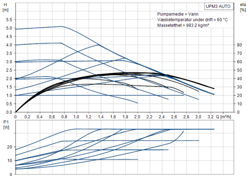
Pumpekurve UPM3 25-50:
