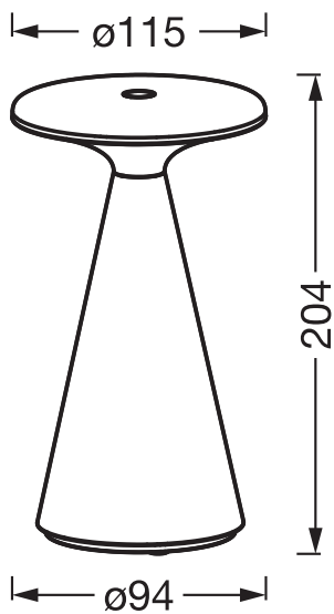
SMART BT TABLE LUM TWIST RGBW IP44
