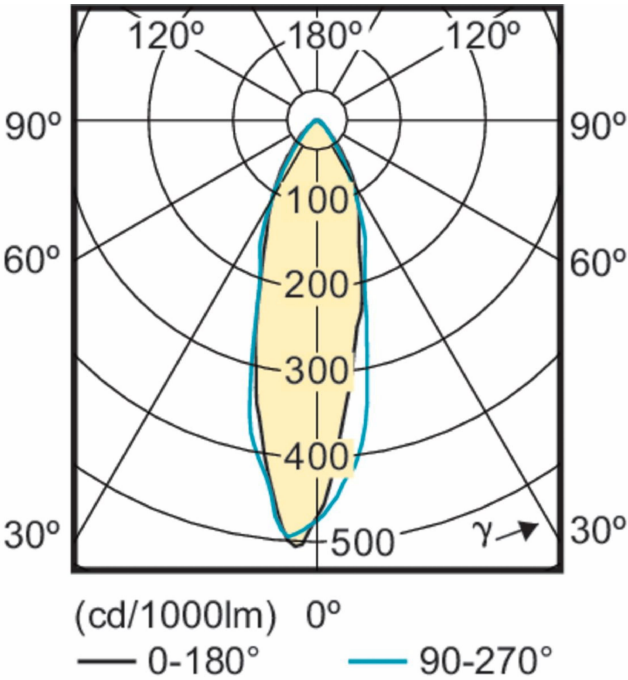
Light Distribution Diagram - Corepro LEDspot 2.7-25W GU10 827 36D
