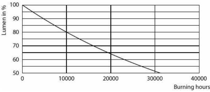
Lumen Maintenance Diagram - MAS VLE LEDBulbD11.2-100W E27 927 A60FRG
