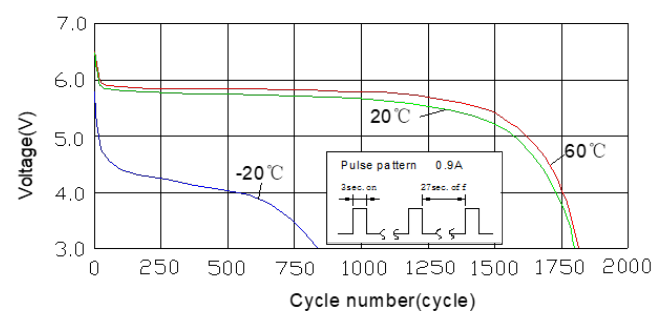
Pulse discharge characteristics
