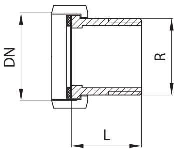
External thread tailpieces
