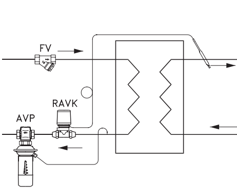
Heat exchanger in radiator heating system
