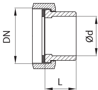
Weld-on tailpieces
