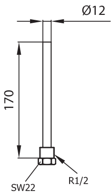
Immersion pockets
