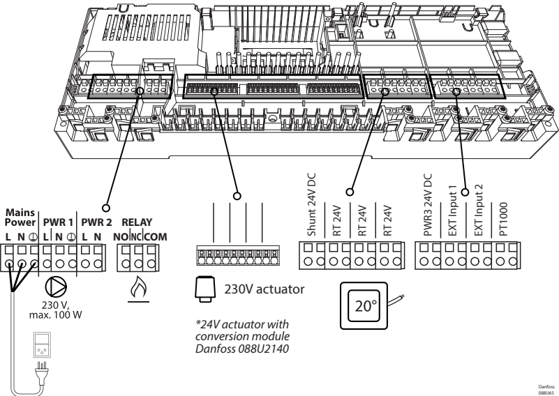
Figure: Danfoss Icon2™ Main Controller connection
