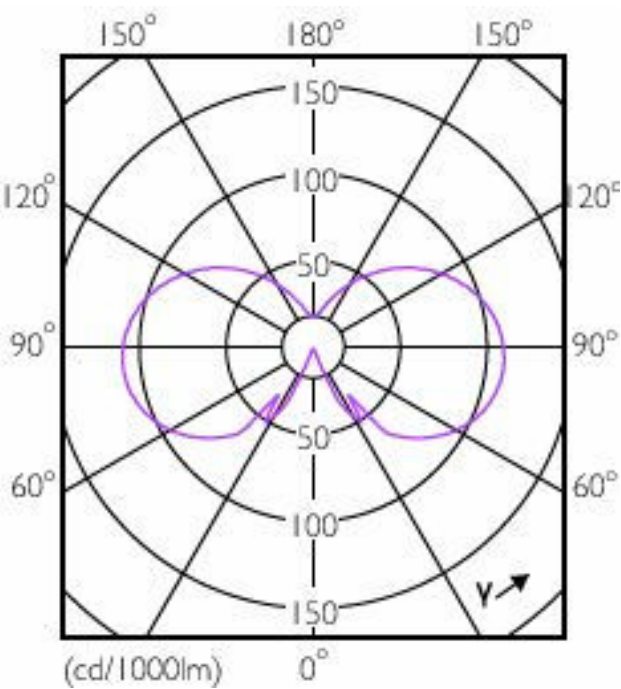
Light Distribution Diagram - CorePro LEDLusterND4.3-40W E27 827P45CLG
